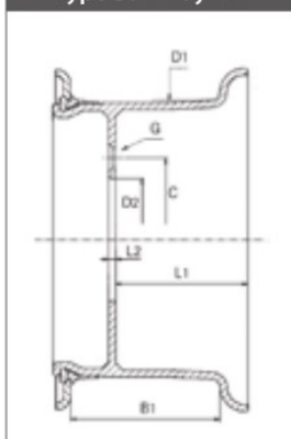
Type D: 4-way rim
