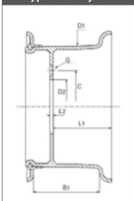
Type C: 3-way rim
