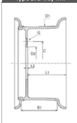
Type D: 4-way rim
