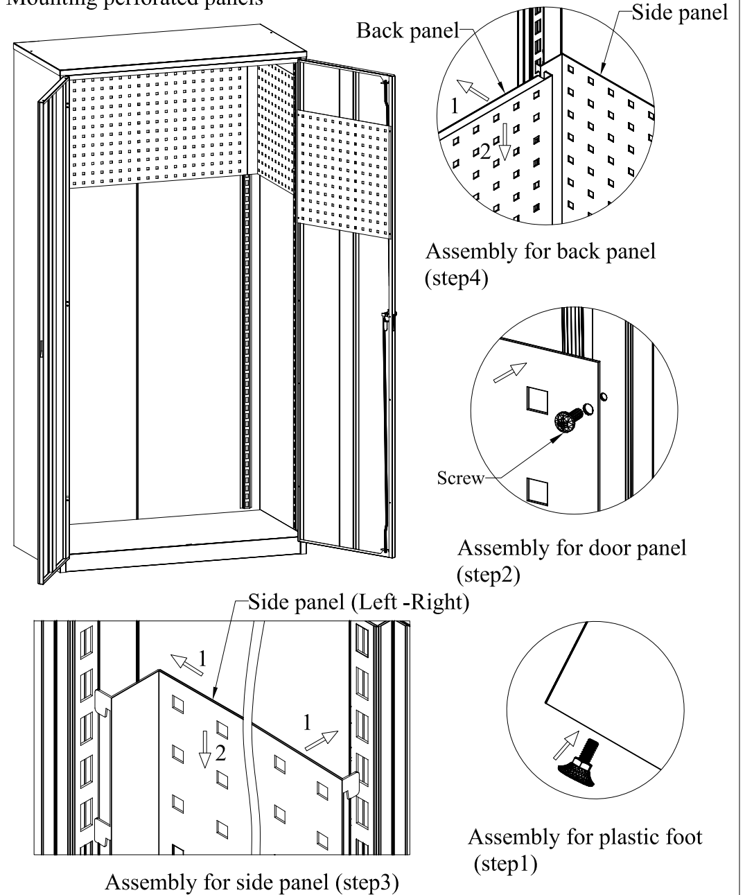
Mounting perforated panels
