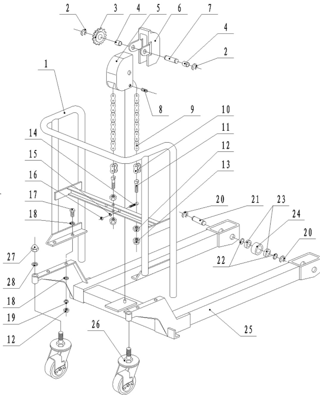
Figure 3 Frame Assembly
