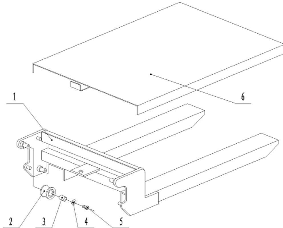
Figure 1 Packet Bracket Assembly
