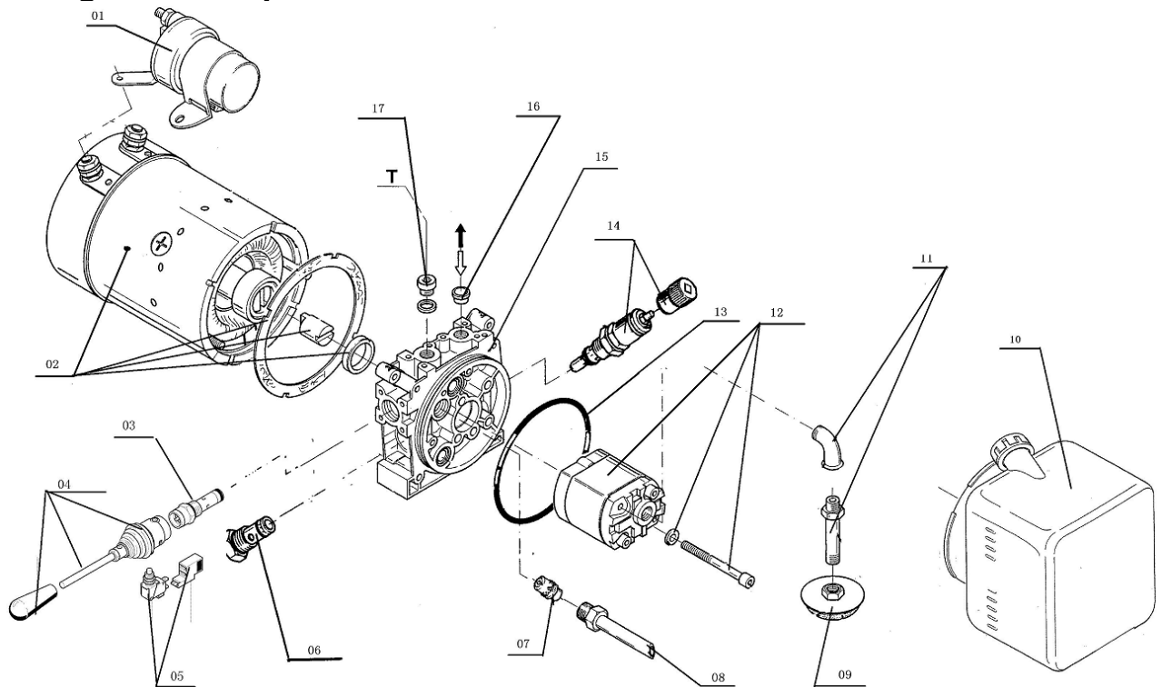
Figure 6 Pump Station Parts
