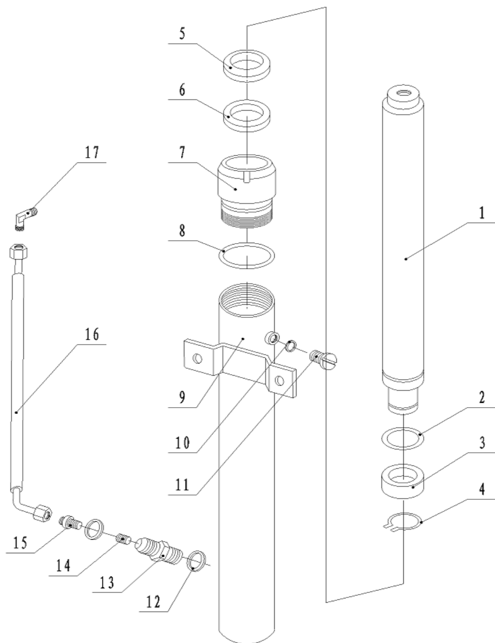
Figure 7 Oil Tank Components
