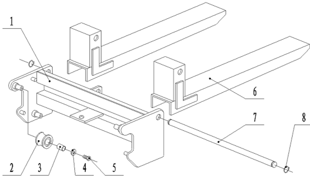
Figure 2 Portable Packet Bracket Assembly
