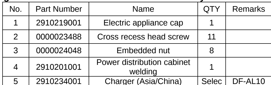
Figure 4 Power Distribution Cabinet Assembly
